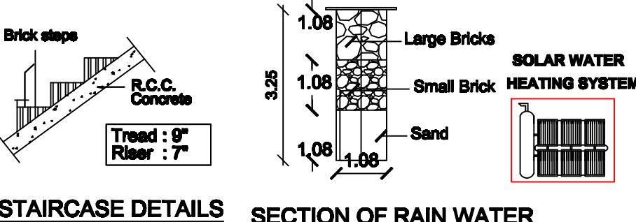
STAIRCASE DETAILS
