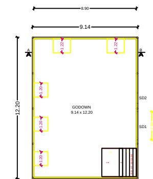
GROUND FLOOR PLAN (SOUTH FACING)
