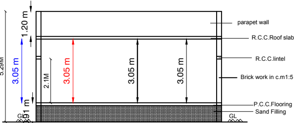
SECTION-"SR"
