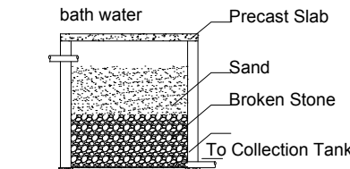
Section of Filter Unit
