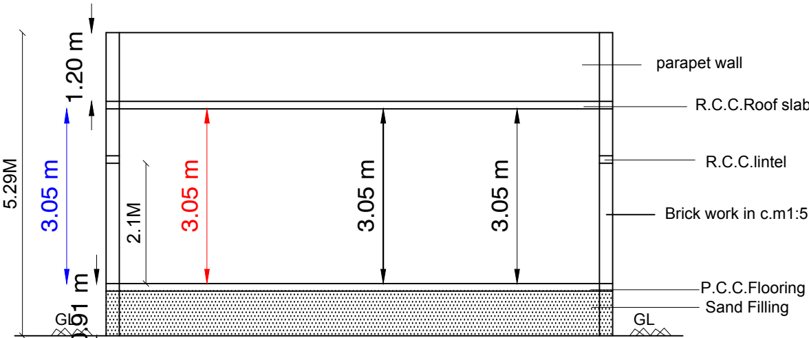
SECTION-"SR"
