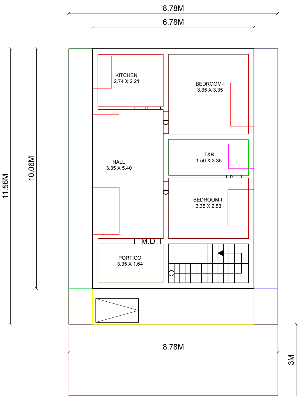
GROUND FLOOR
