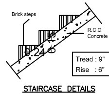
STAIRCASE DETAILS
