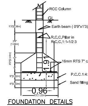
FOUNDATION DETAILS
