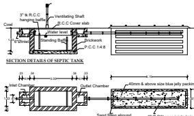
DETAILS OF SEPTIC TANK & DISPERSION TRENCH
