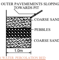
RAIN WATER PERCOLATION BED
