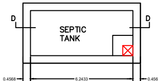
PLAN OF SEPTIC TANK SCALE 1"=2'0"
