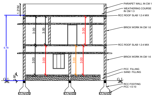
SECTION ON S-R
