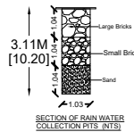
SECTION OF RAIN WATER COLLECTION PITS (RWC)
