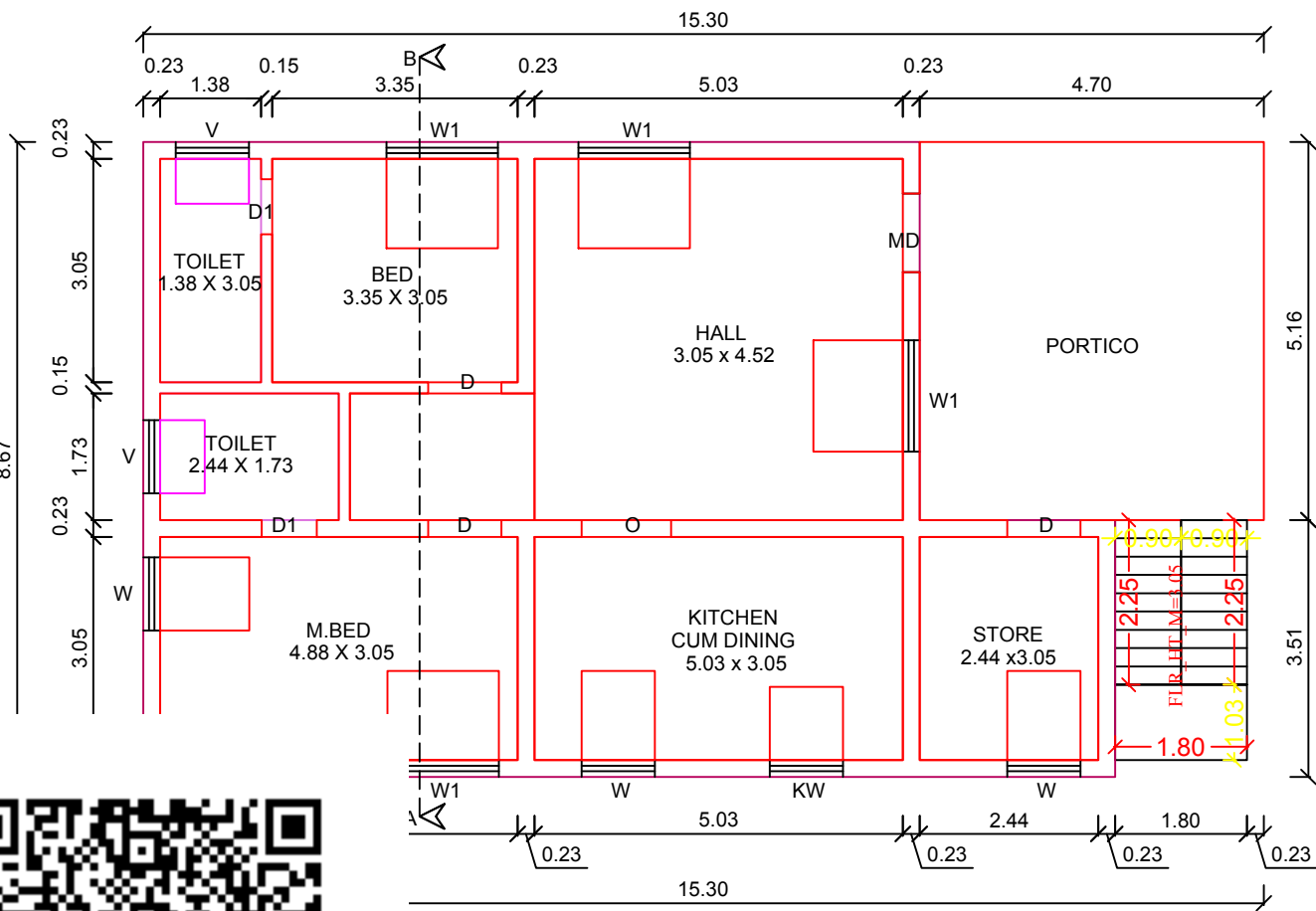
O.GROUND FLOOR PLAN
