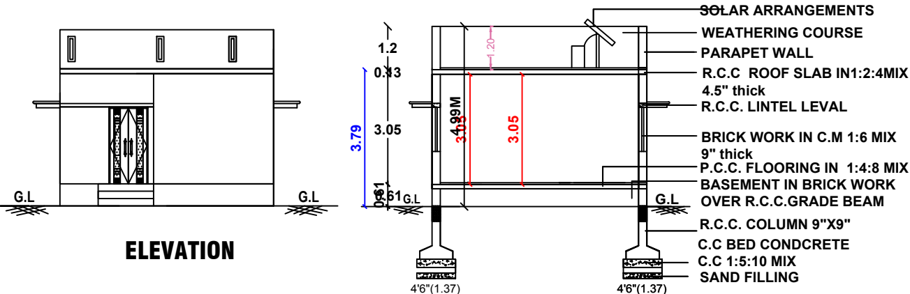
SECTION " AB "
