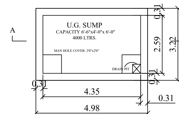
SUMP DETAIL
