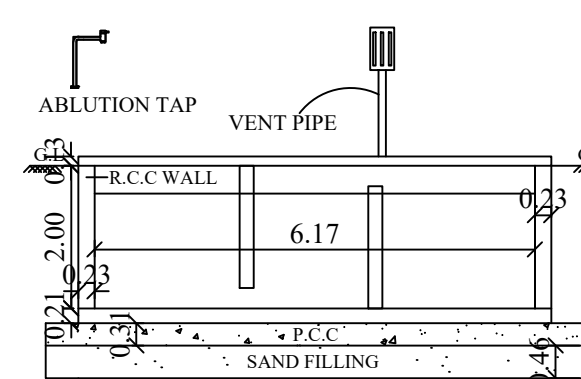
SECTION ON K-B
