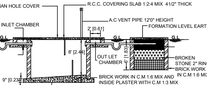
SECTION OF SEPTIC TANK AND DISPERSION TRENCH
