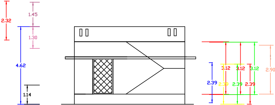
FRONT ELEVATION
