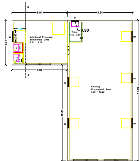
PLAN - Ex . & Additional Proposed Ground Floor - commercial Building
