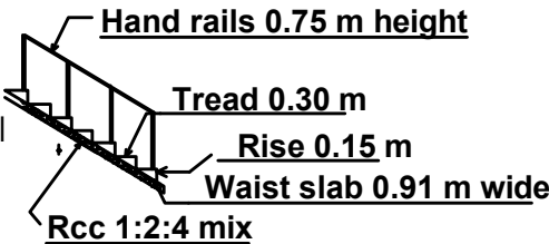
Staircase Details
