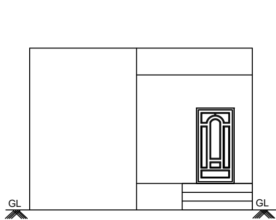
FRONT ELEVATION (EAST FACING)
