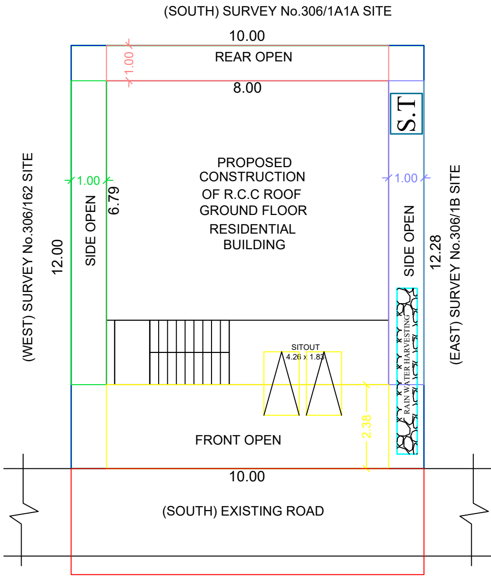
SITE PLAN
