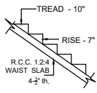
STAIRCASE DETAILS (NTS)
