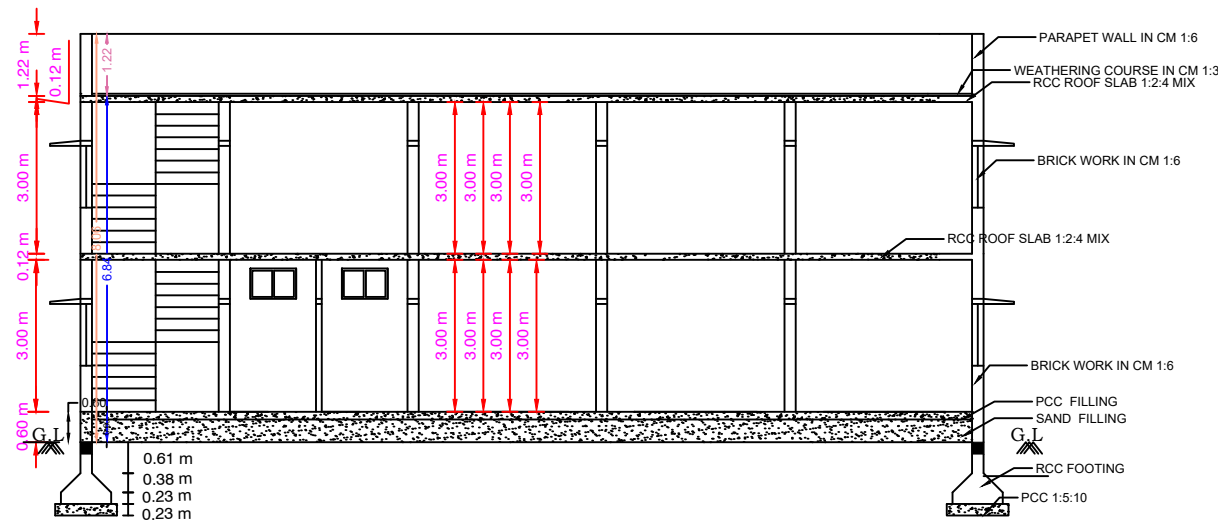
SECTION ON KA
