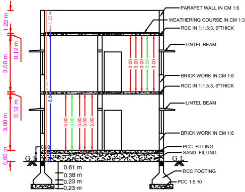
SECTION OF KA
