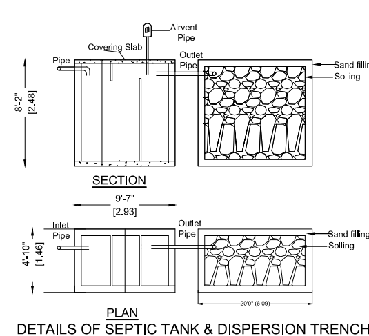
DETAILS OF SEPTIC TANK & DISPERSION TRENCH
