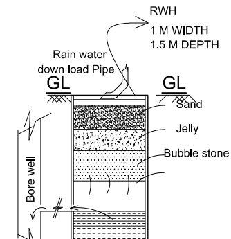
SEC. RAIN WATER HARVEST PIT
