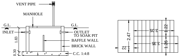
SECTION OF SEP.TANK
