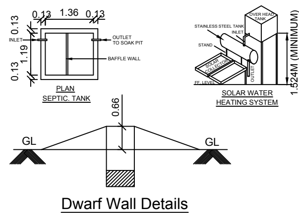
SOLAR SYSTEM
