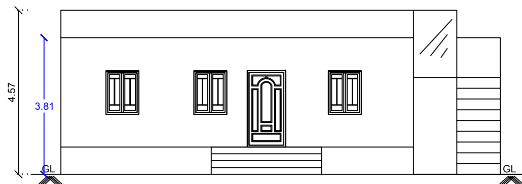
FRONT ELEVATION (EAST FACING)
