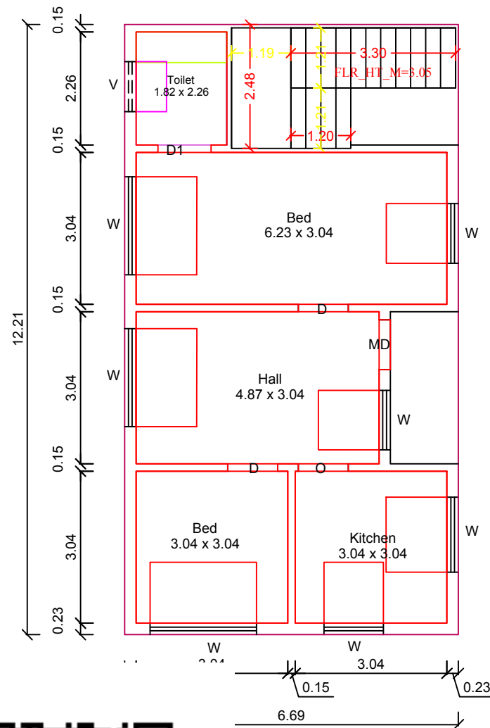
ND FLOOR PLAN
