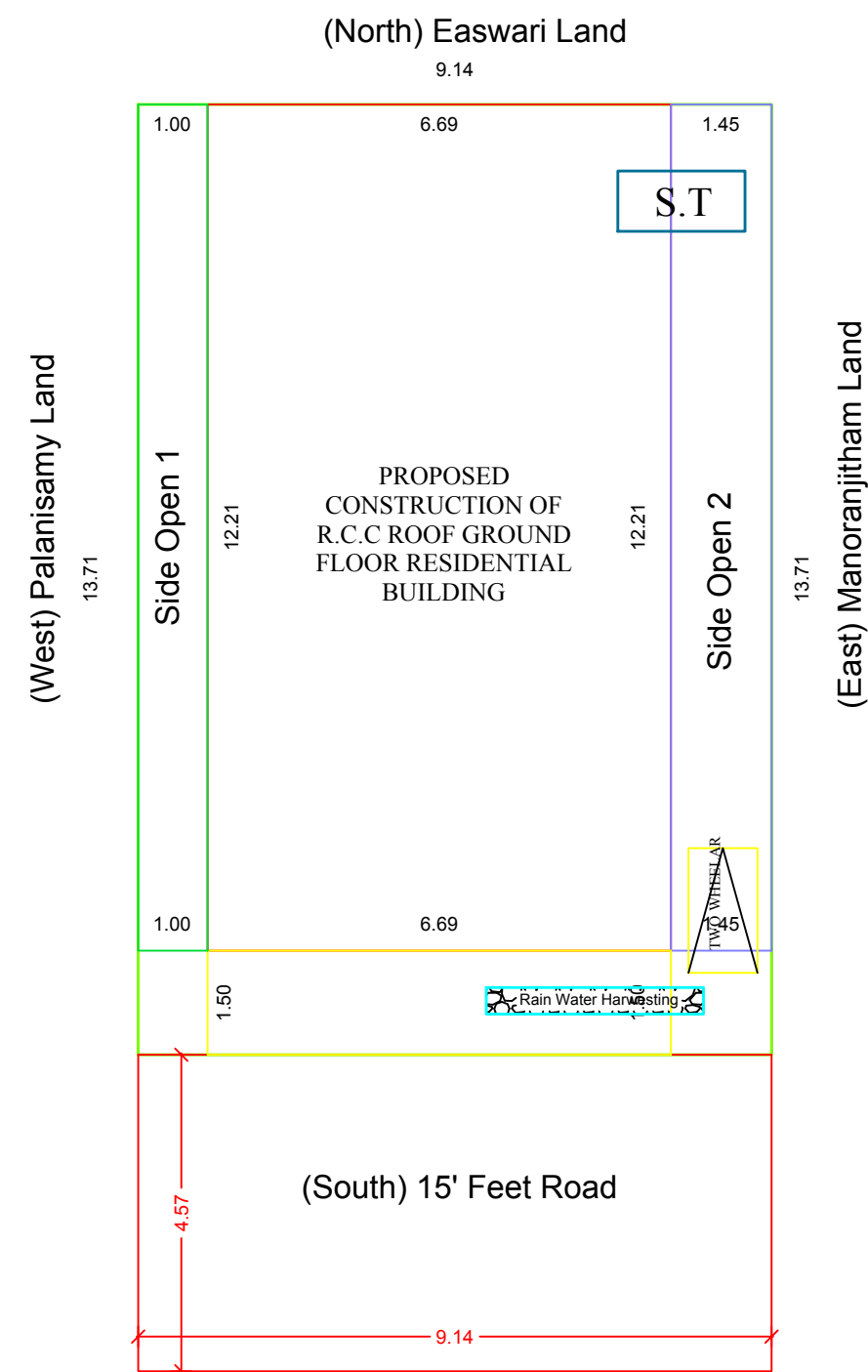
SITE PLAN
