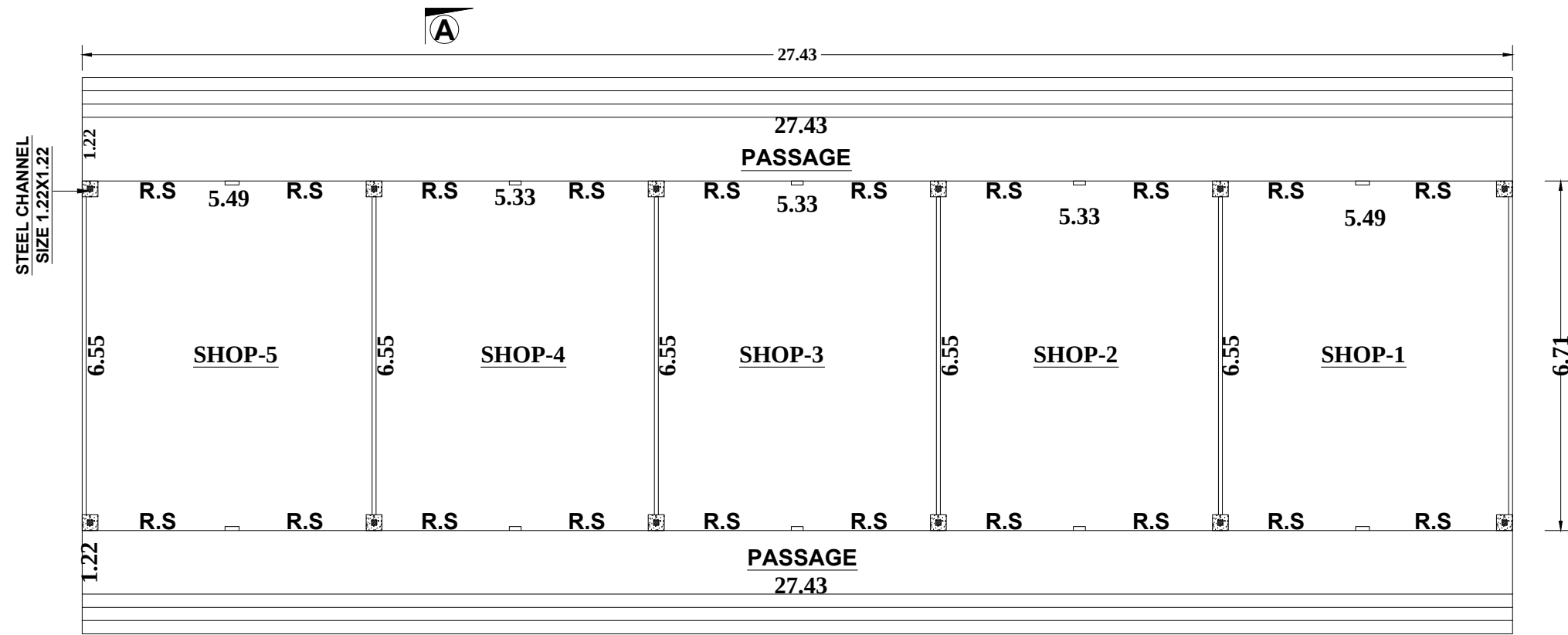
.GROUND PLAN .
