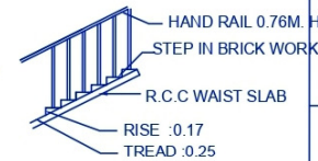
STAIR CASE DETAIL
