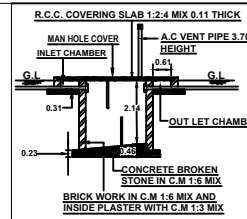
SECTION ON SEPTIC TANK .
