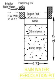
RAIN WATER PERCOLATION PIT
