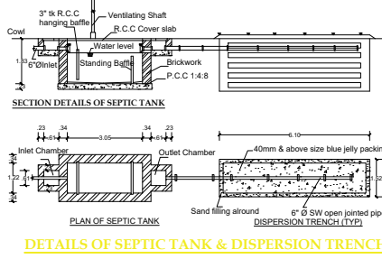
DETAILS OF SEPTIC TANK & DISPERSION TRENCH
