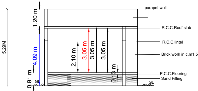
SECTION-"SR"
