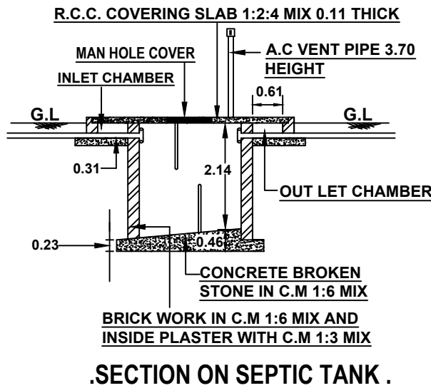
SECTION ON SEPTIC TANK .
