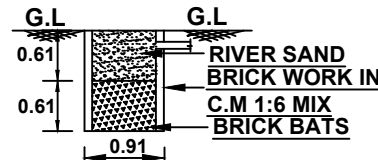
SECTION ON RAIN WATER COLLECTION TUB .
