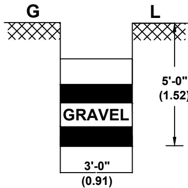
TRIAL PIT (NTS)
