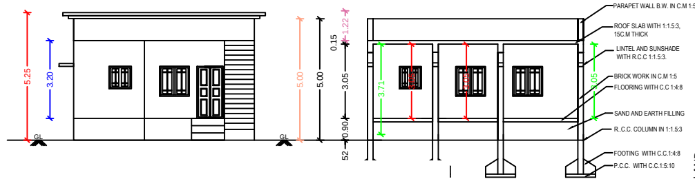
ELEVATION ON AB
