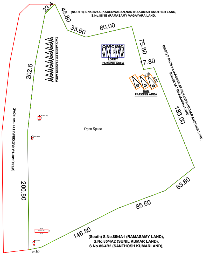
SITE PLAN SITE PLAN NOT TO SCALE
