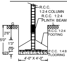
FOUNDATION DETAIL
