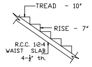
STAIRCASE DETAILS (NTS)
