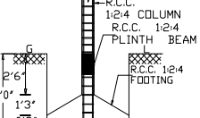
FOUNDATION DETAIL
