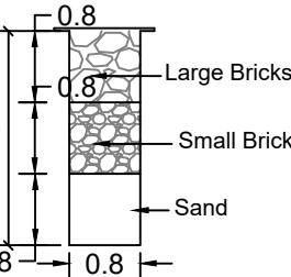
SECTION OF RAIN WATER COLLECTION PITS (NTS)
