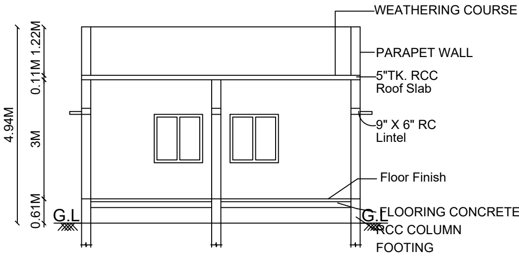
SECTION ON 'SP'
