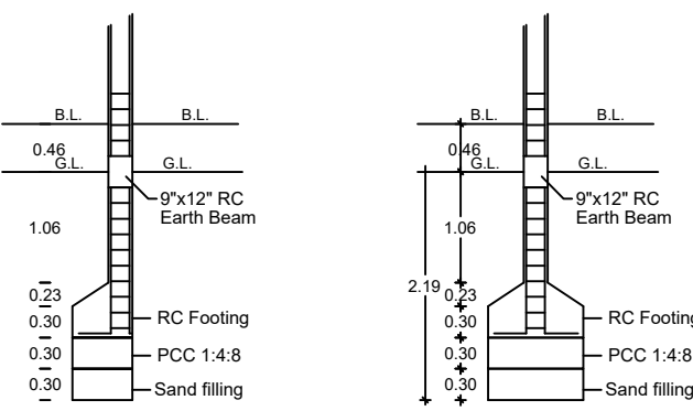
FOUNDATION DETAILS (ONE SIDE FOOTING)
