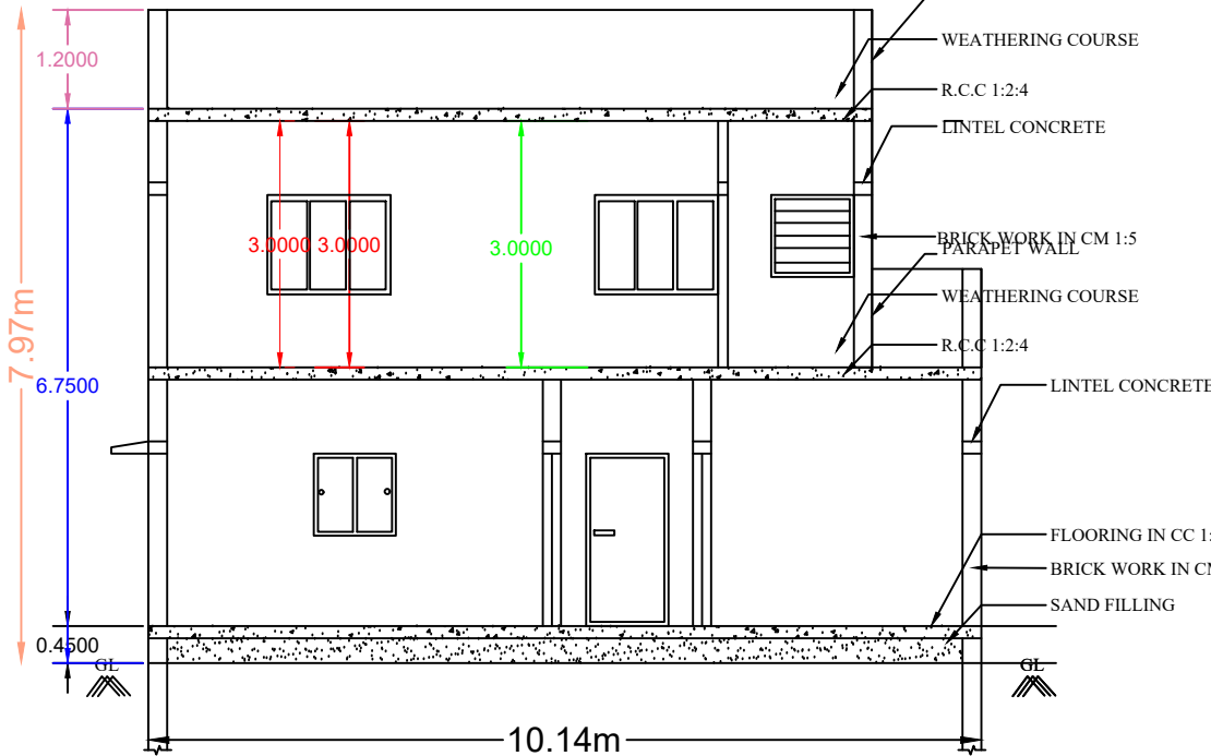
SECTION AA
