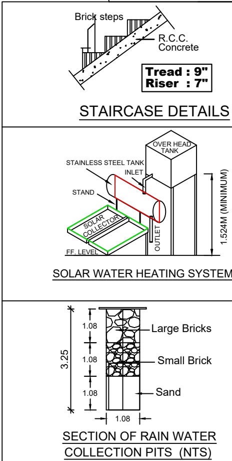
SECTION OF RAIN WATER COLLECTION PITS (NTS)
