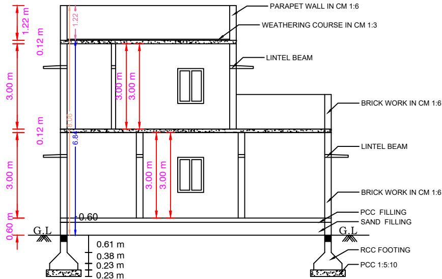
SECTION ON KA
