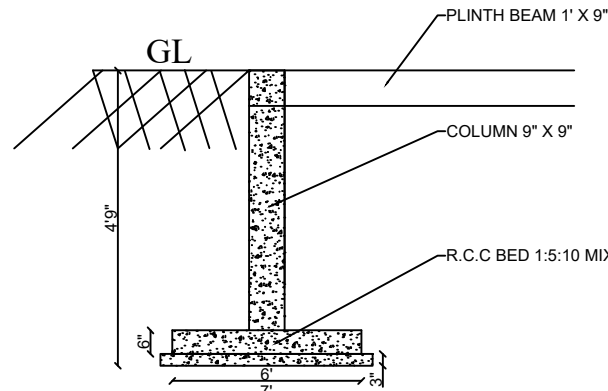
FOOTING DETAILS
