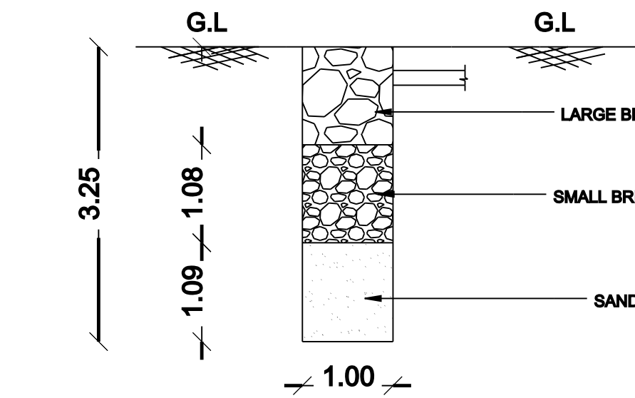
SECTION OF RAIN WATER HARVESTING PIT
