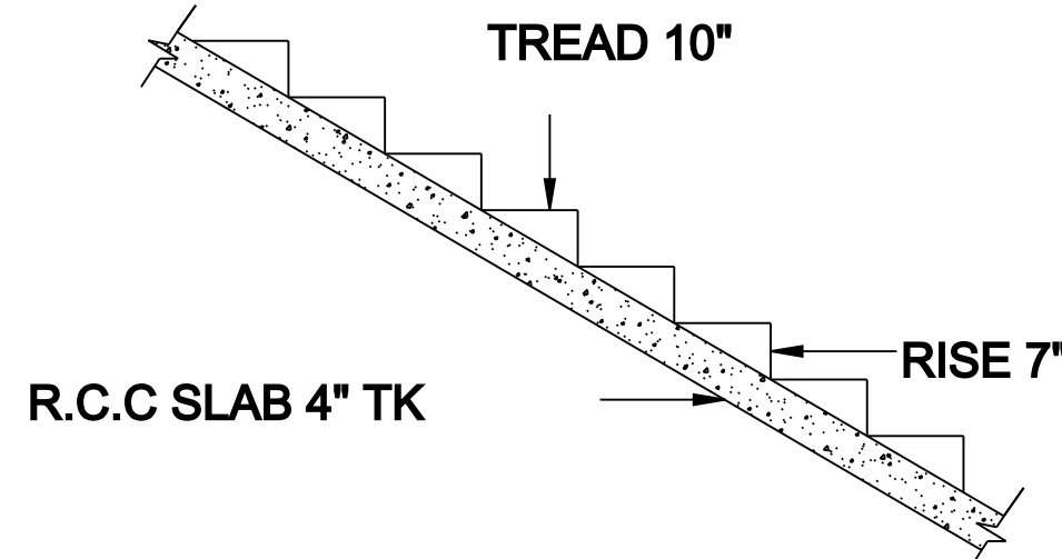
STAIRCASE DETAILS
