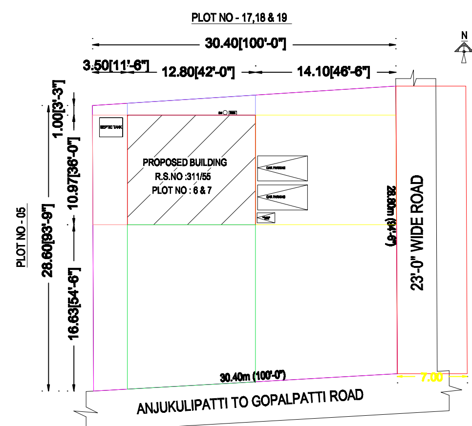
SITE PLAN
