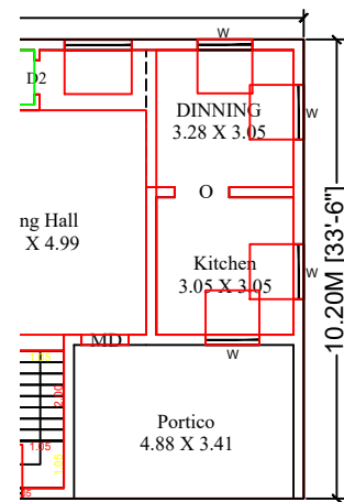
2 FLOOR PLAN
