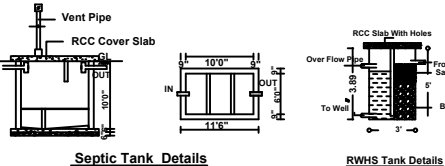
Septic Tank Details
