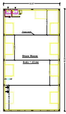
Proposed Ground Floor Plan - Store Room
