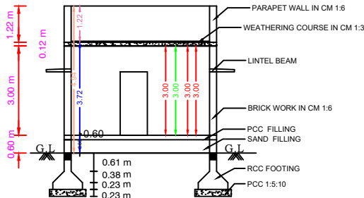
SECTION ON KA
