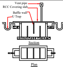
Waste Water Recycle Unit
