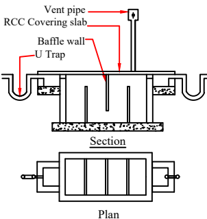
Septic Tank With U Trap
