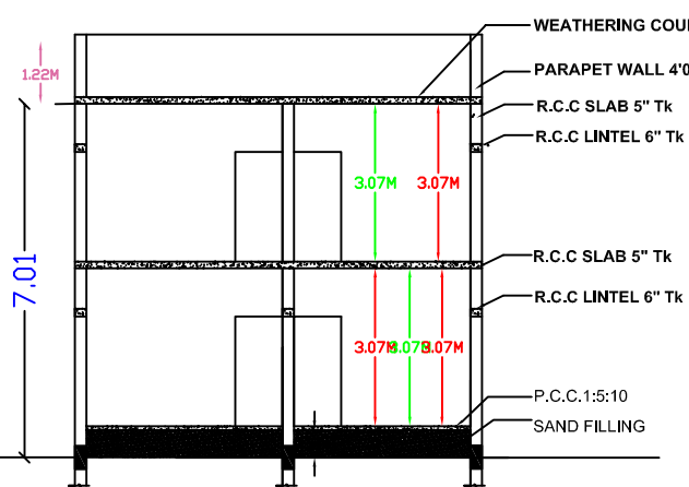
Section - AA Section
