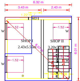
FIRST FLOOR COMMERCIAL
