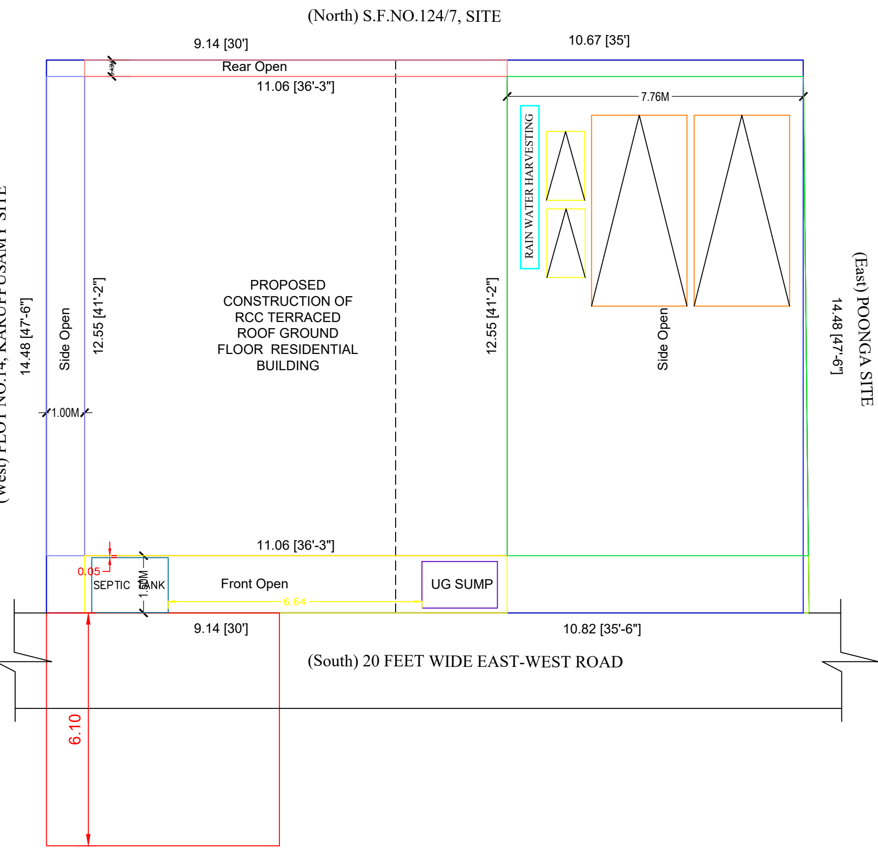
SITE PLAN
