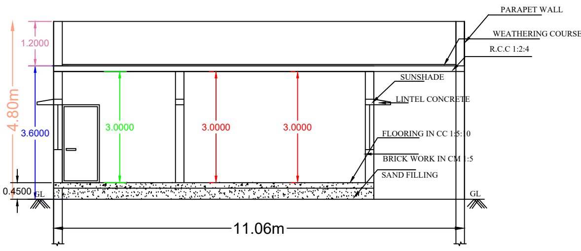
SECTION AB
