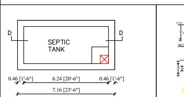
PLAN OF SEPTIC TANK SCALE 1"=2'0"
