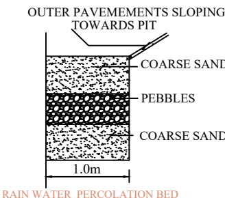
RAIN WATER PERCOLATION BED
