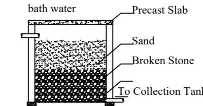
Section of Filter Unit
