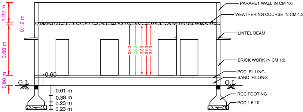
SECTION ON KA
