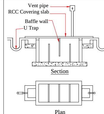
SECTION - 'CD'
