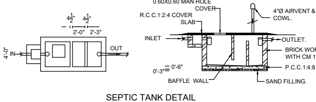
SEPTIC TANK DETAIL
