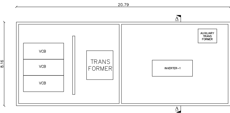
PLAN OF INVERTER BLOCK-B
