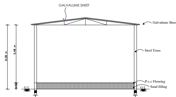
TYPICAL SECTION OF INVERTER BLOCK-B
