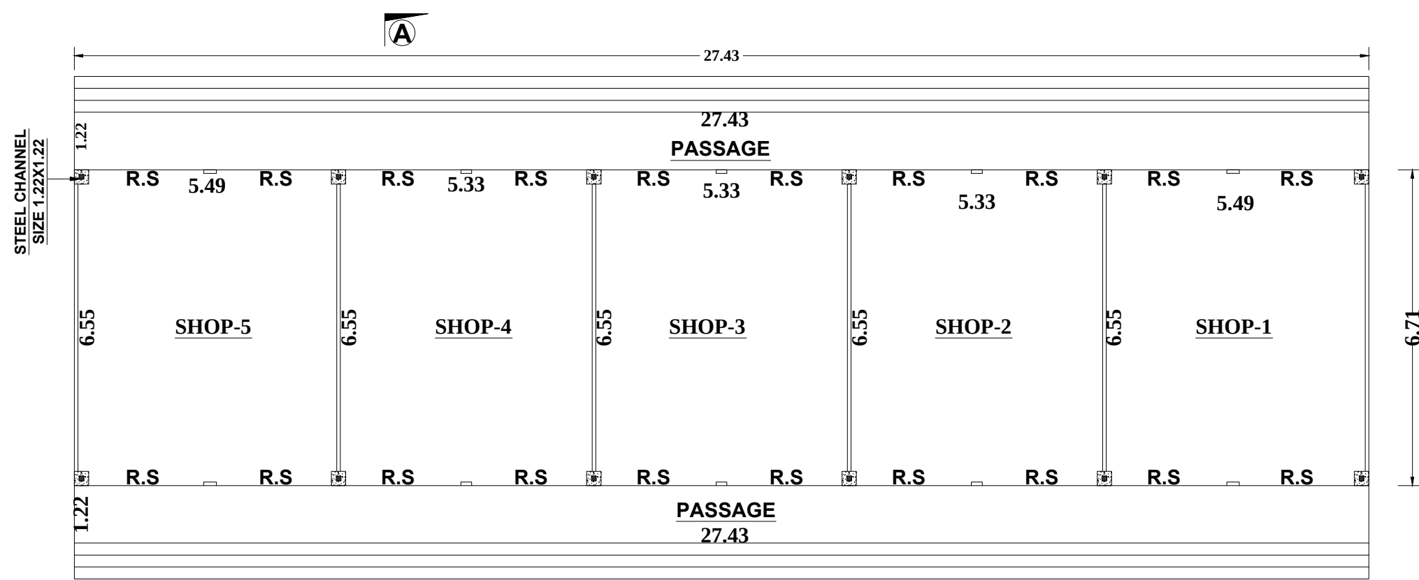
.GROUND PLAN .
